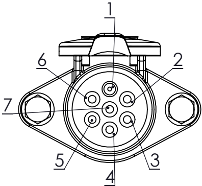
Conector PQ macho 7 vias
